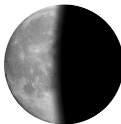
Last quarter
