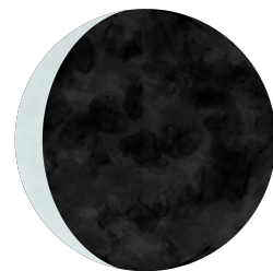
Waning crescent
