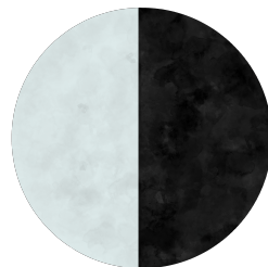
Last quarter
